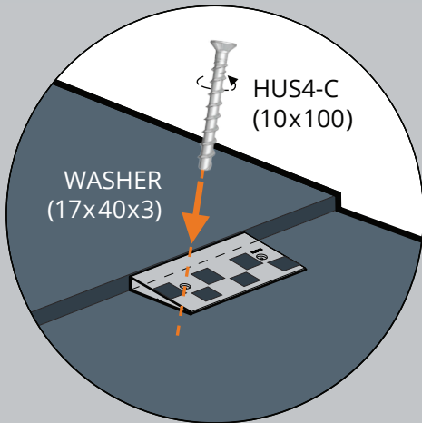
screw
