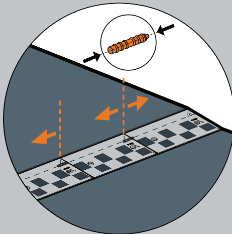
plug - repeat
